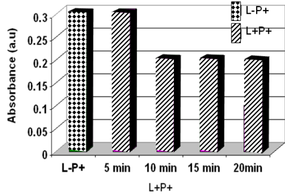
Fig. (3): Absorption spectroscopic measurements for malachite green (0.025mg /ml) after irradiation with 650nm diode laser.
